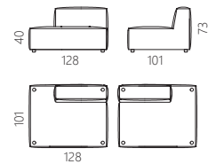
ID : 3009-55F 3009-56F open end/LHF open end/RHF
