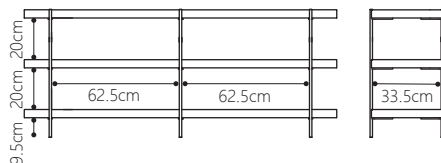
HUMLA 152 low shelf W152.5 D34.5 H62.5 cm
